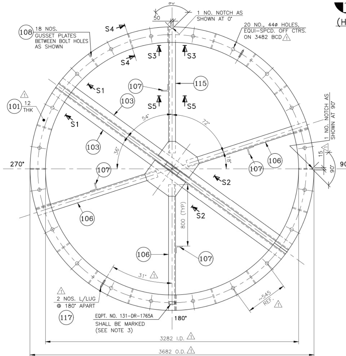
PLAN VIEW DETAIL OF BASE RING TEMPLATE FOR SITE (QTY. REQD.: 2 NO.)
